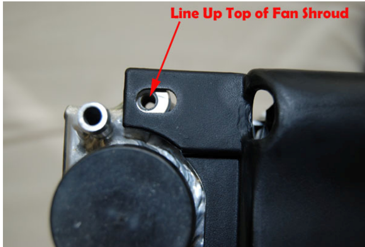
Picture 1: Line up the top of the fan shroud to match mounting hole
